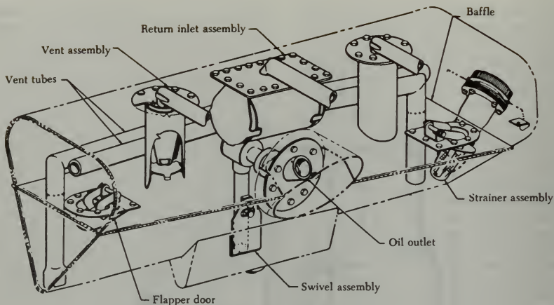
FIGURE 6-23. Oil tank.
